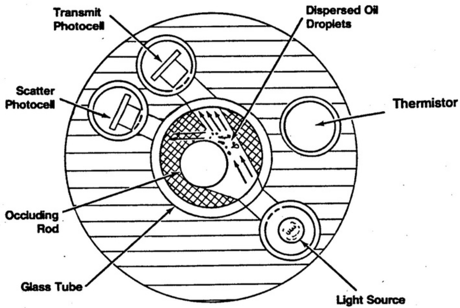
Cross Section of Sensing Head
