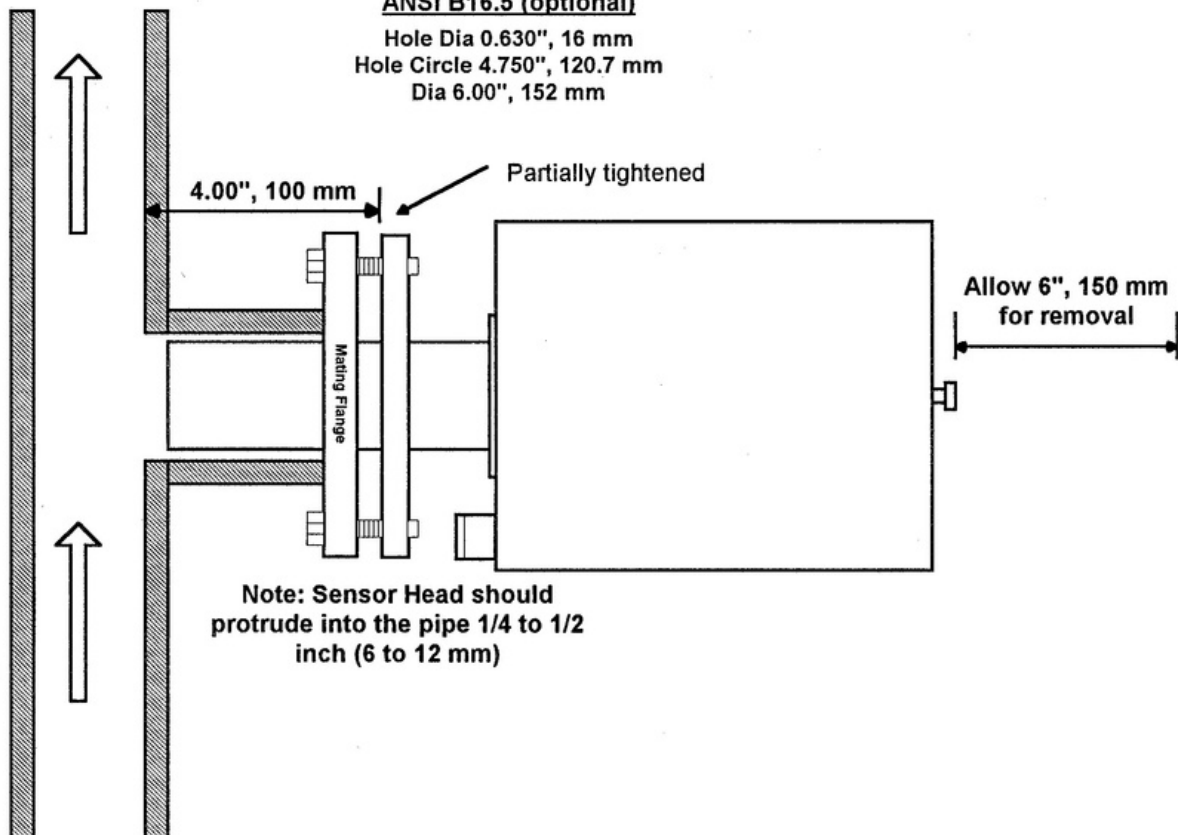
Figure 2 BA-200 Installation 23
