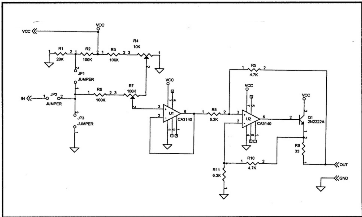
CL001 4-20mA Schematic
